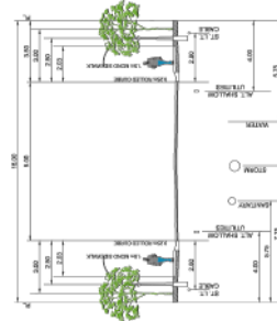
RESIDENTIAL STREET "M-L" 9.0m/16m
