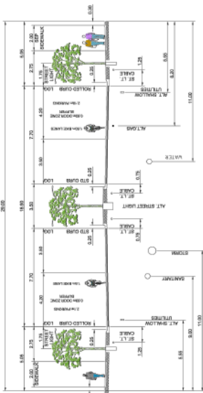
3. Modified 10.8m/22.0m COLLECTOR Belvedere Point SE
