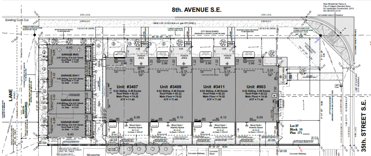
Figure 3: Site Plan
