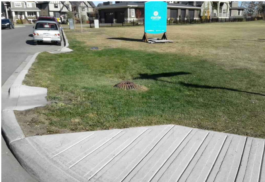
Bioretention – along Beny-Sur-Mer Road SW
