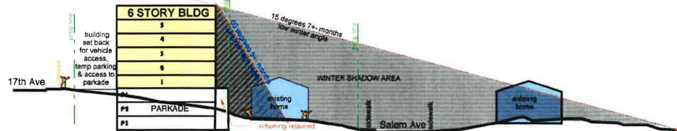
6 STORY BUILDING SUN SHADOWS WINTER + SUMMER SECTION THROUGH PROPOSED UPZONED AREA ON 17TH AVE SW
