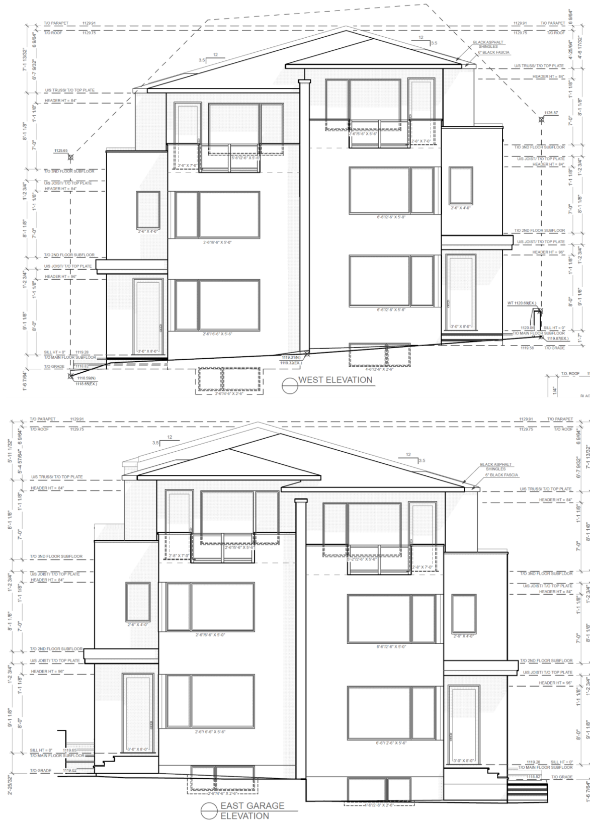
Figure 3: Elevations
