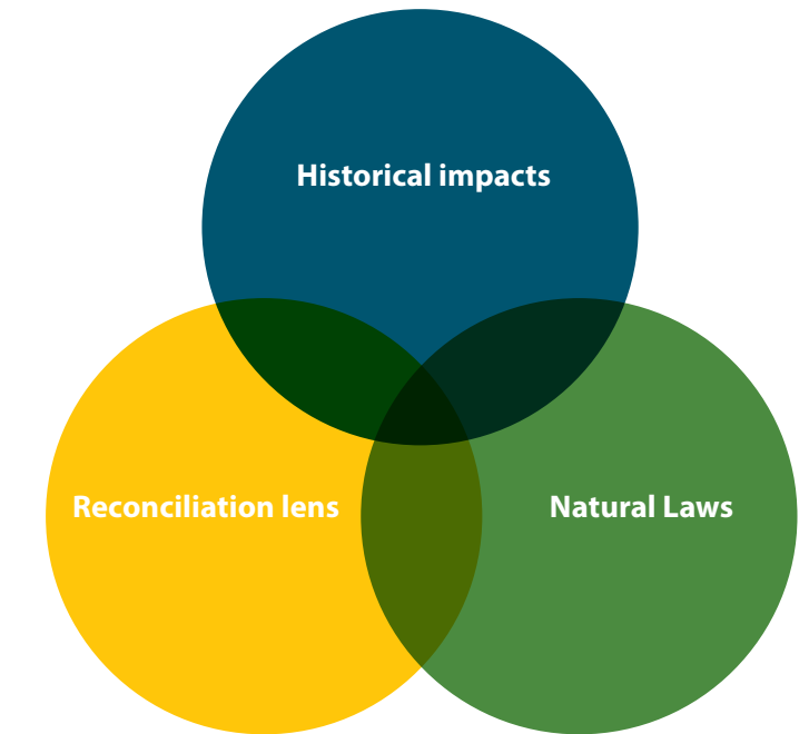
Figure 2: Key frames
