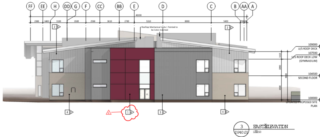
Figure 3 – East Elevation (Facing the Laneway)
