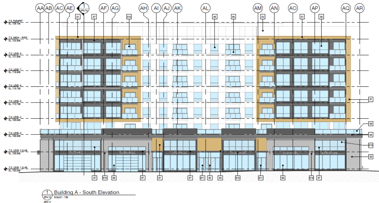
Figure 3: Proposed south elevation of Building A
