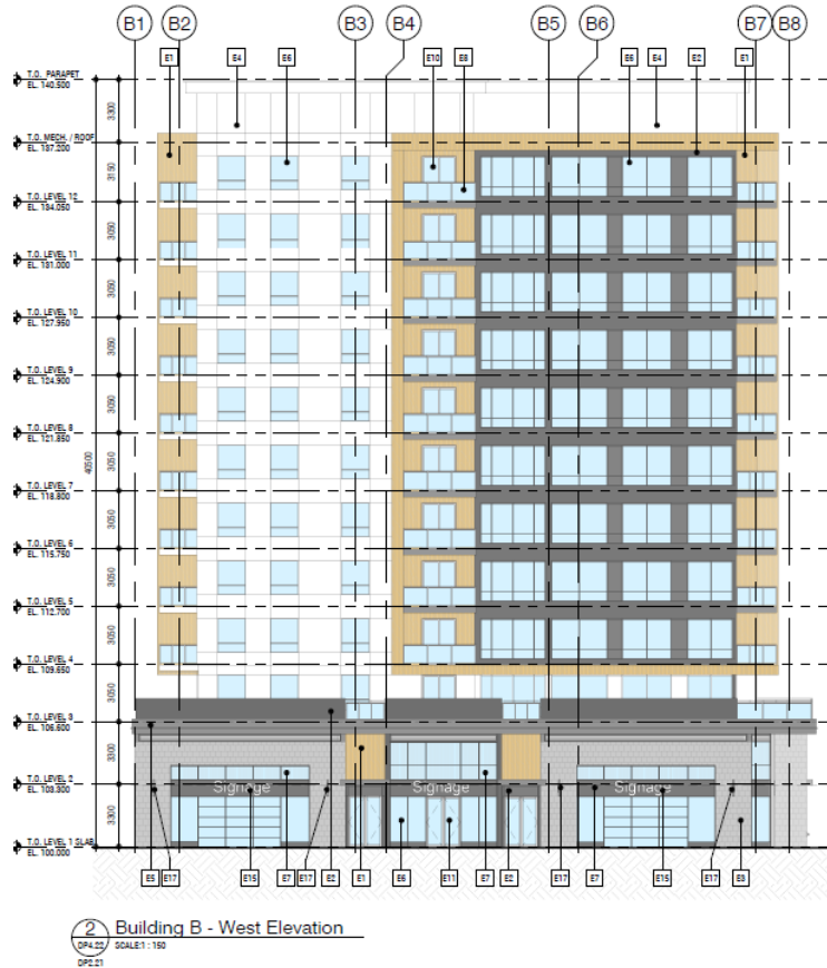
Figure 4: Proposed west elevation of Building B
