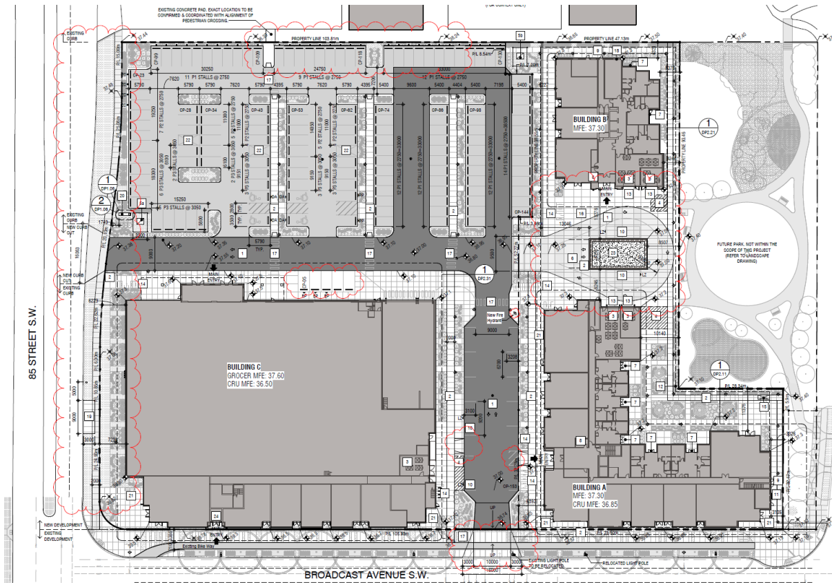
Figure 2: Proposed site layout and landscaping plan
