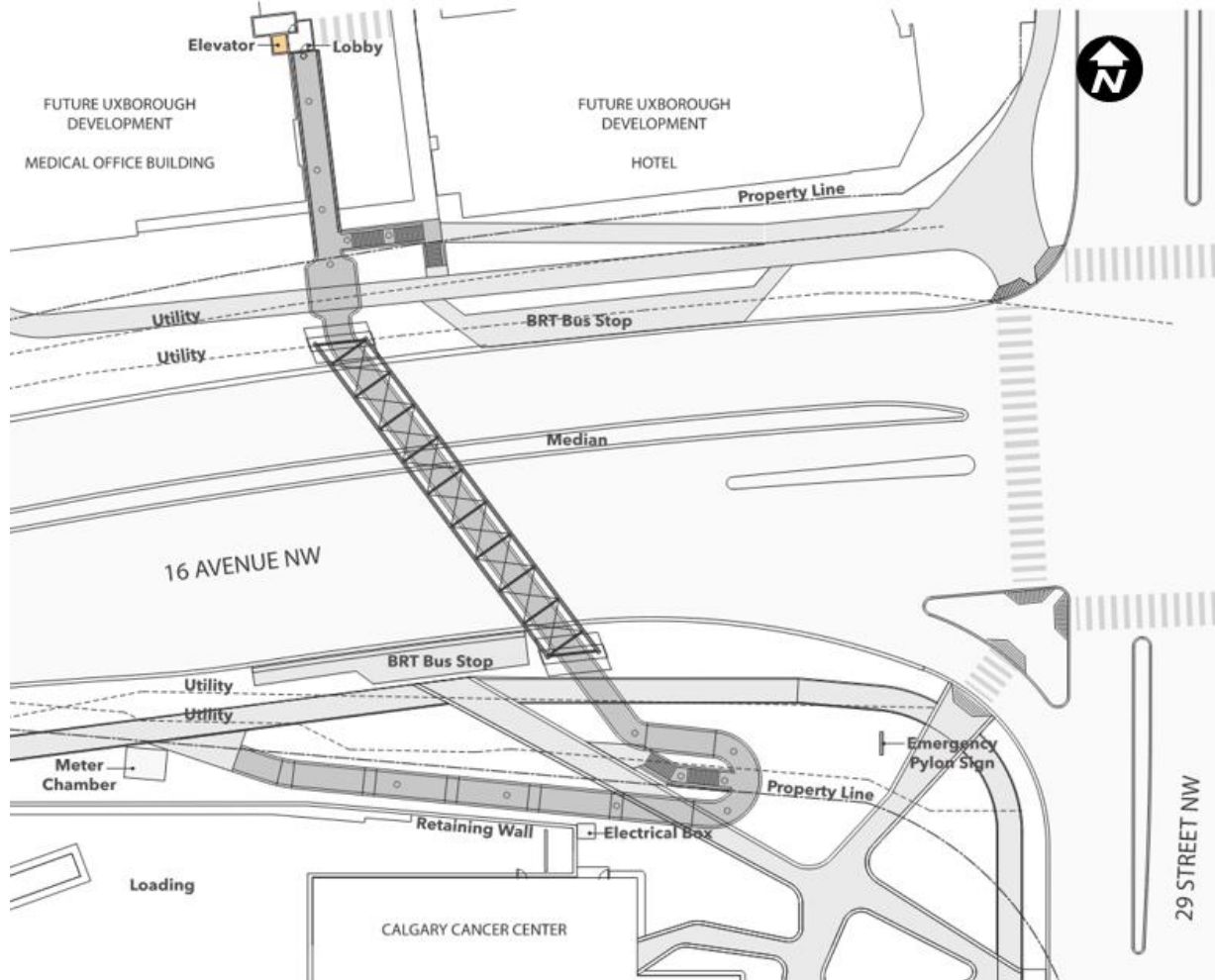
Figure 14: Plan View – Pedestrian Overpass
