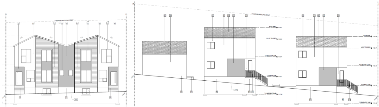
Figure 3: Proposed front elevation of Building A and side elevations
