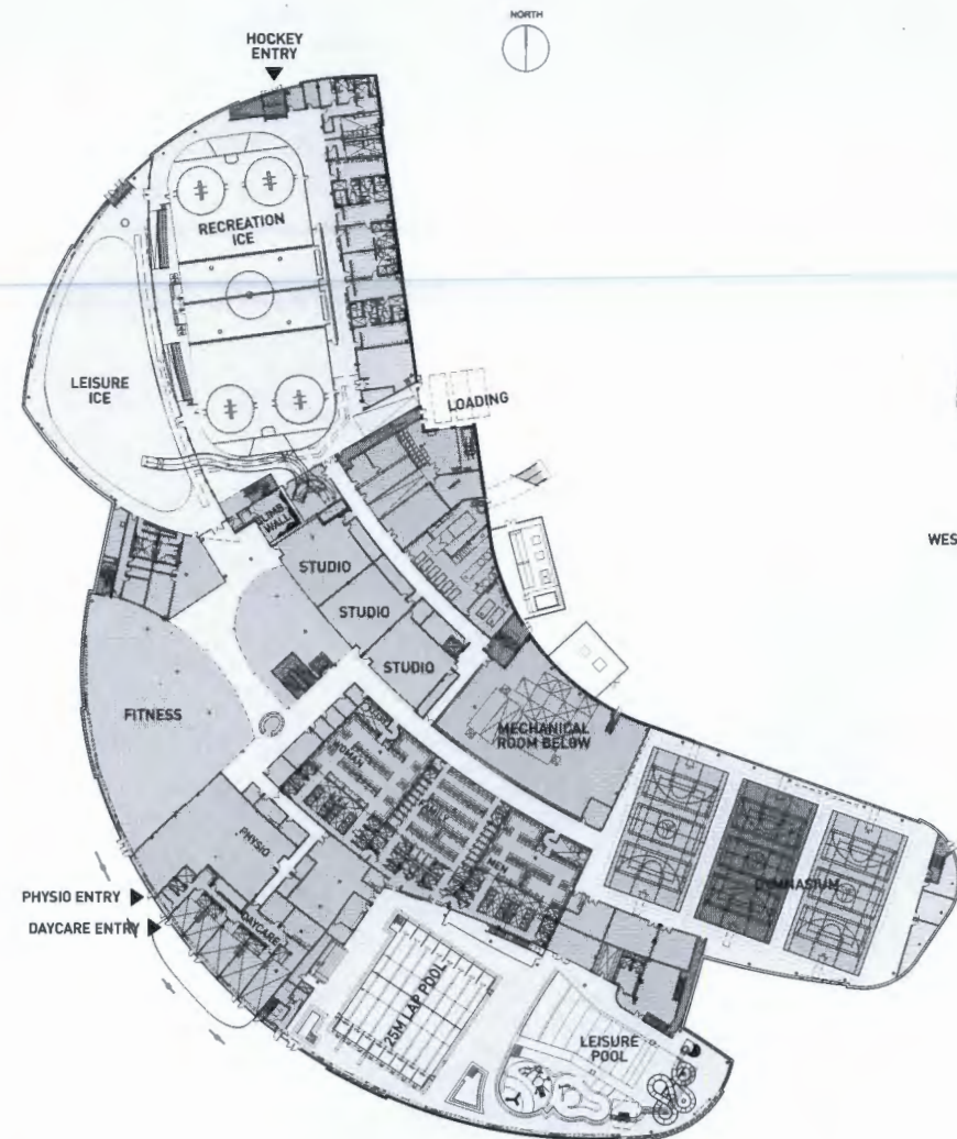
Level One Floor Plan (Activity Level)
