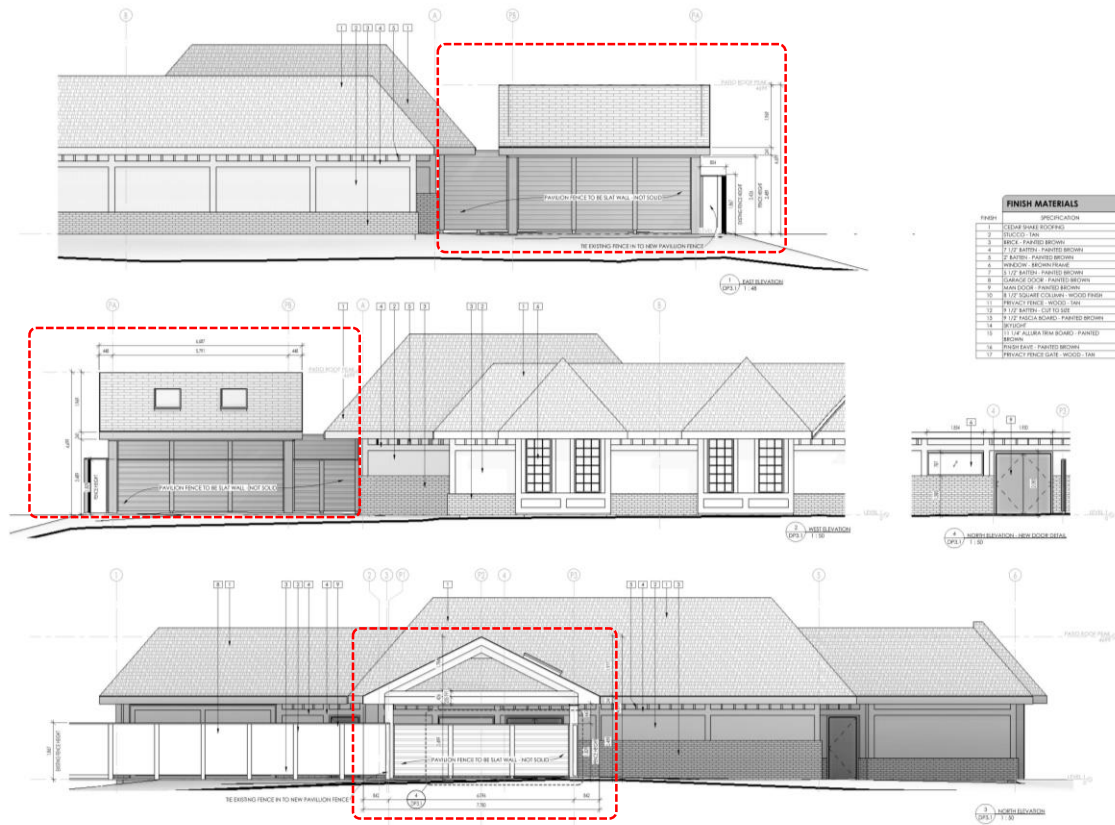
Figure 2: Elevations of Proposed Pavilion
