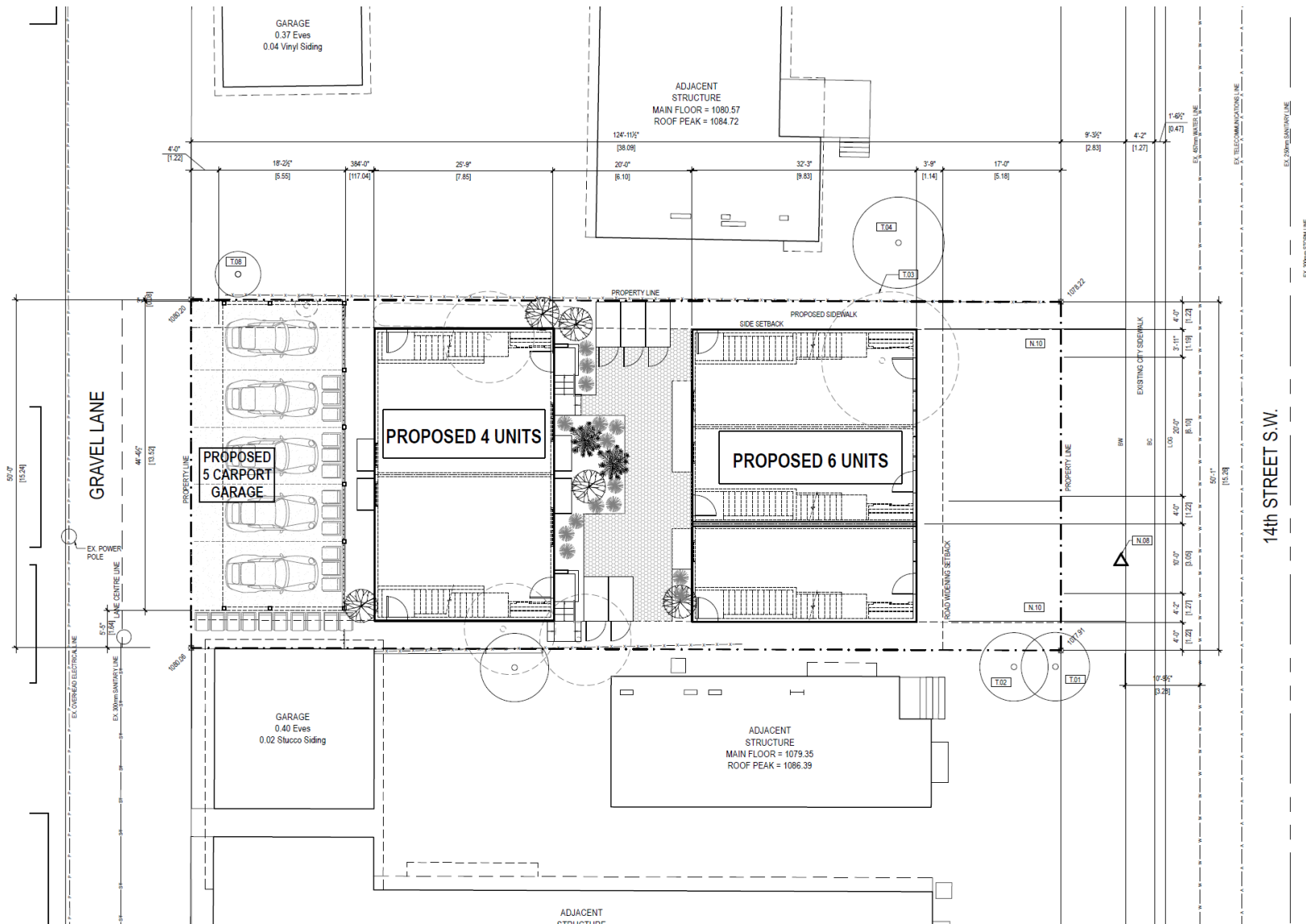
Figure 2: Site Plan
