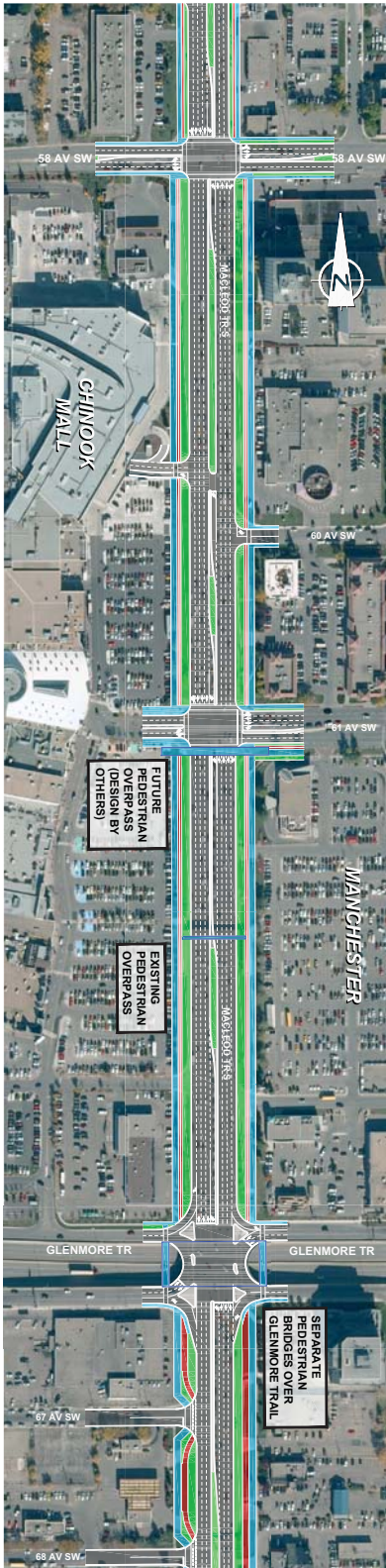
Proposed Urban Boulevard Concept - 58 Avenue S to 67 Avenue S The City of Calgary Macleod Trail Corridor Study 25 Avenue S to 67 Avenue S Figure ES.8
