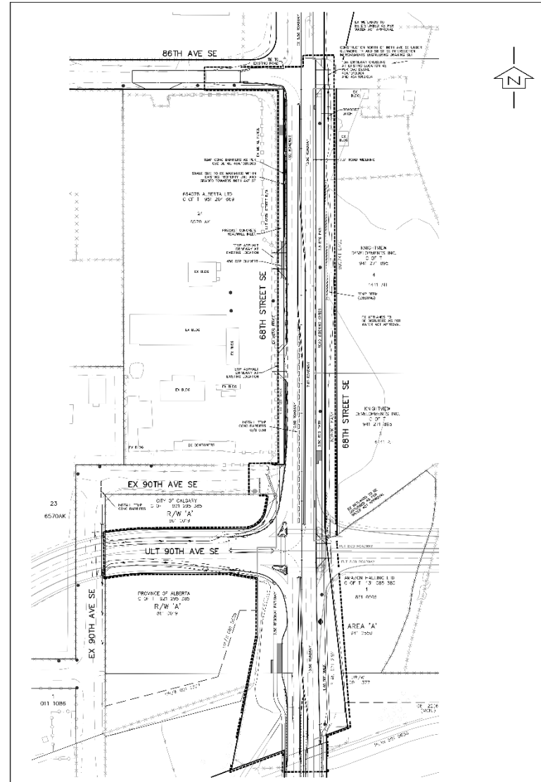
Figure 2 - Road Design
