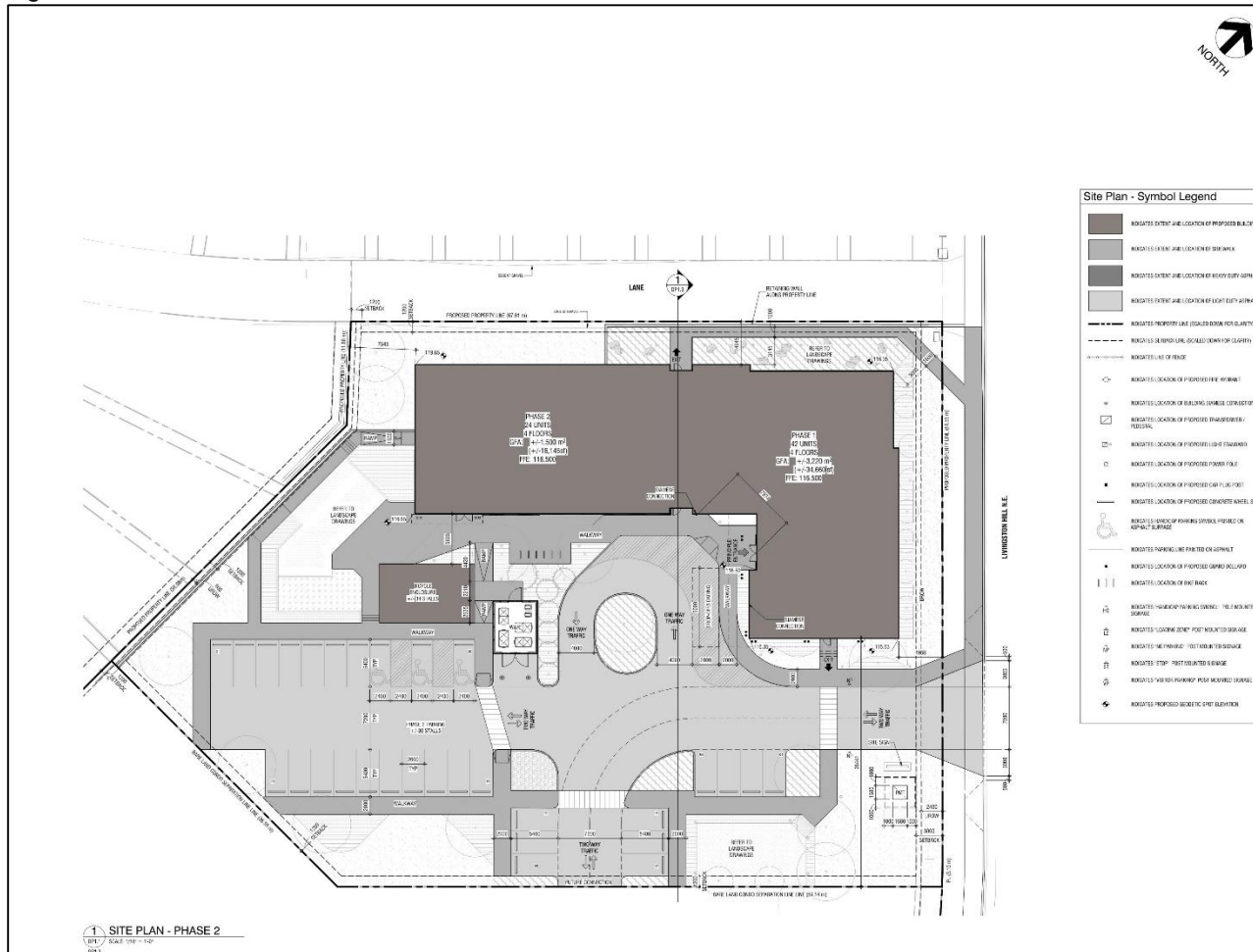
Figure 1: Site Plan
