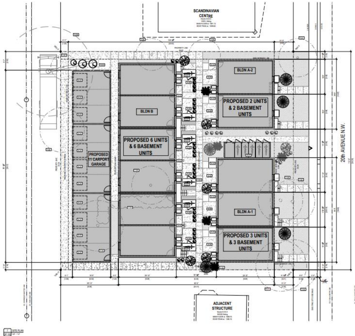
Figure 2: Site Plan of Proposed Development
