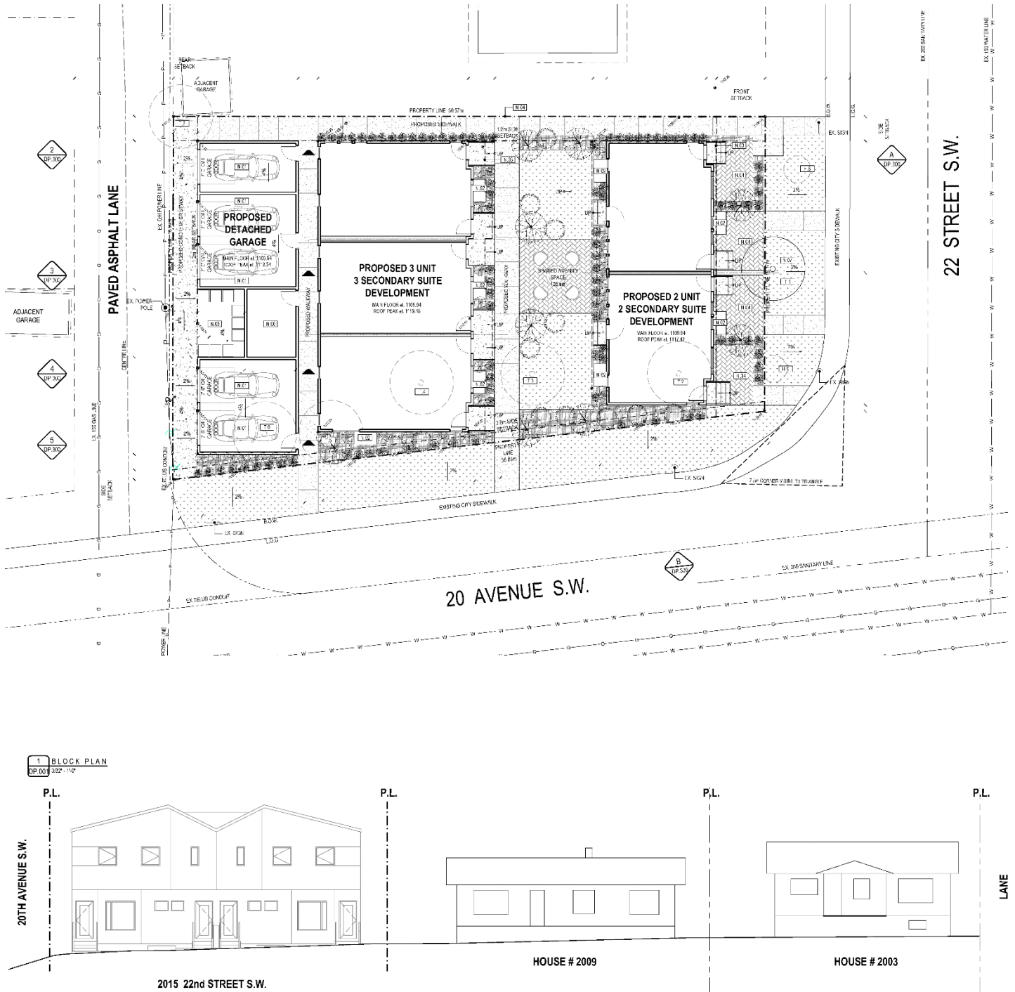
Figure 3: Site Plan and Block Plan
