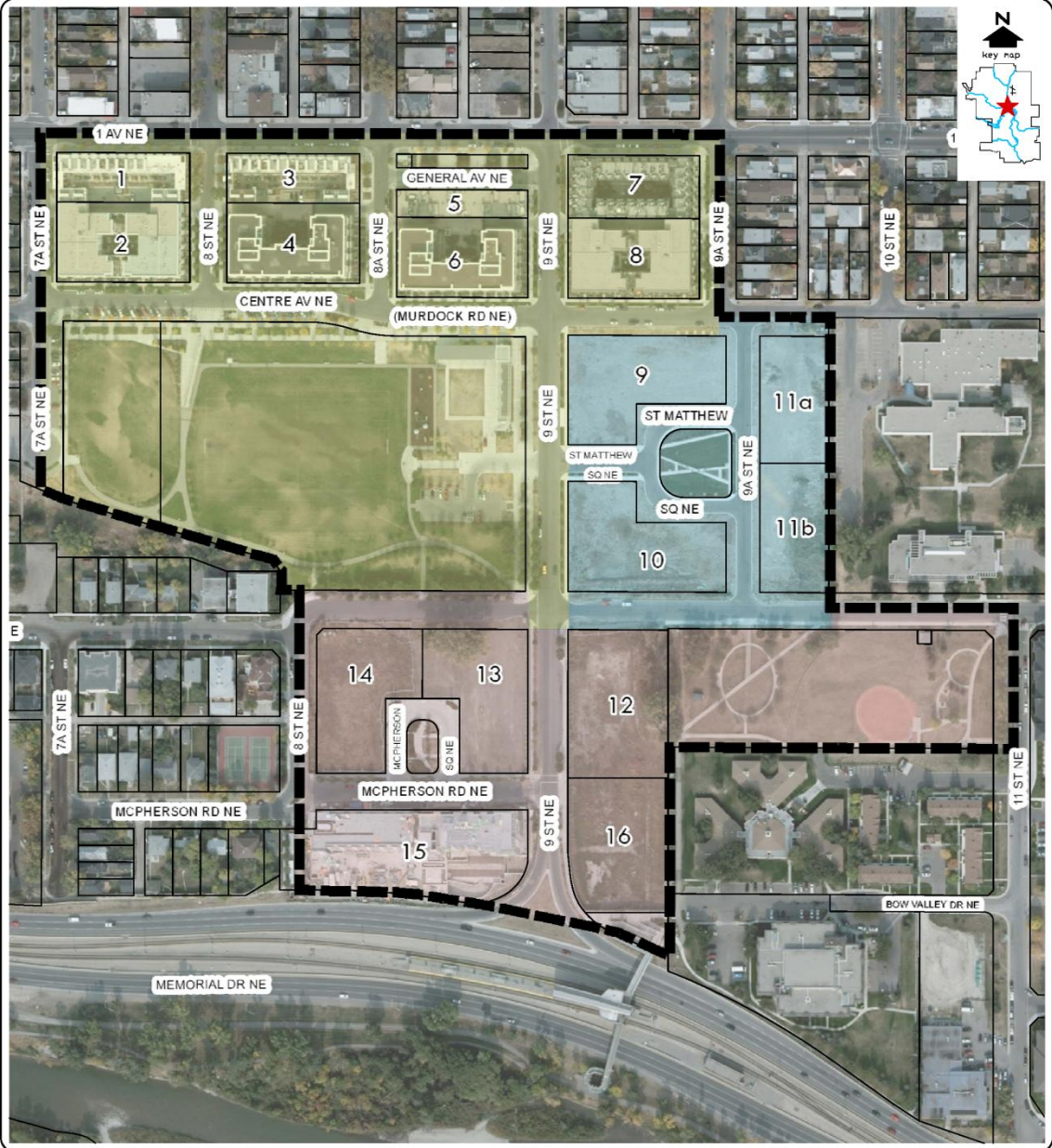
File No. THE BRIDGES - PHASING PLAN (DW)
