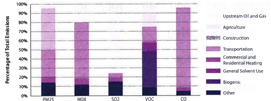
EMISSION SOURCES IN THE CRAZ REGION (2008)
