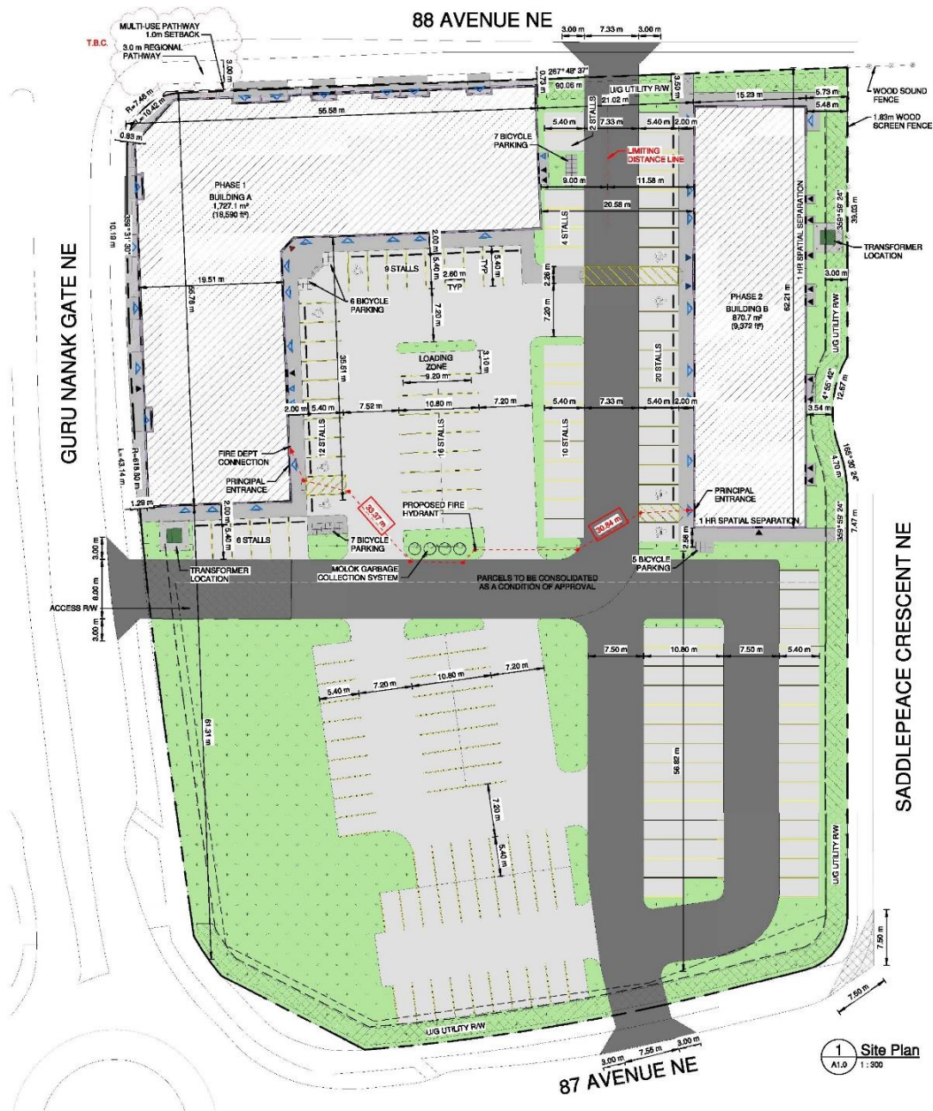
Figure 2: Site Plan
