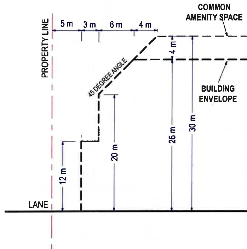
Illustration 1: Building Height in this Direct Control District
