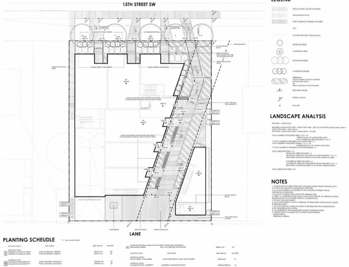
Figure 3: Landscape Plan
