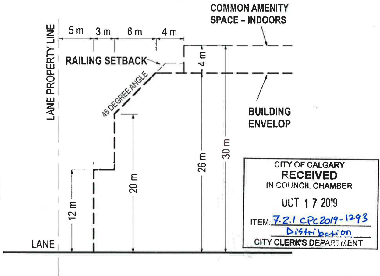
Illustration 1: Building Height in this Direct Control District
