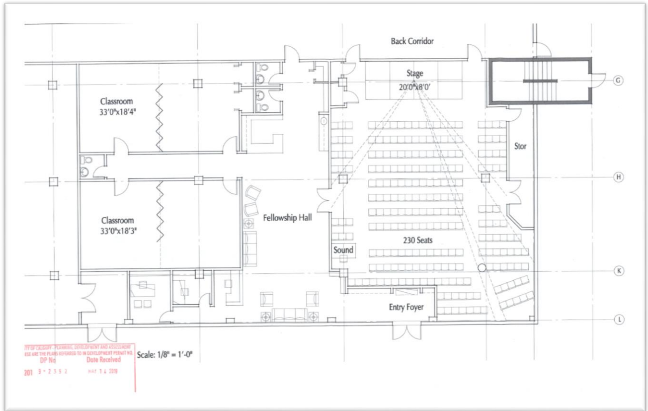
Figure 2: Internal building layout for place of worship
