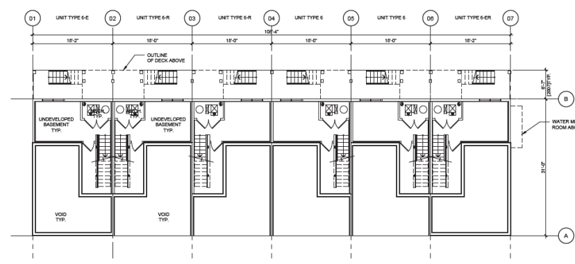
01 BASEMENT FLOOR PLAN DP20-09-01 1/8" = 1'-0"
