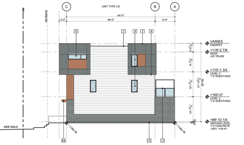
04 WEST ELEVATION DP30-12-01 1/8\" = 1' 0\"
