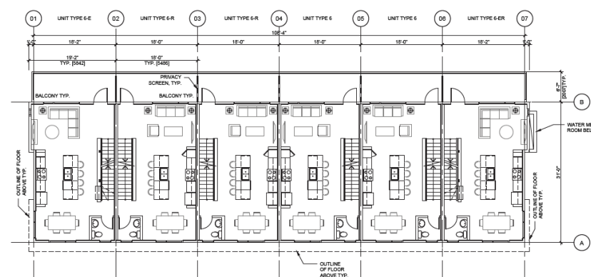
03 SECOND FLOOR PLAN DP20-09-01 1/8" = 1'-0"
