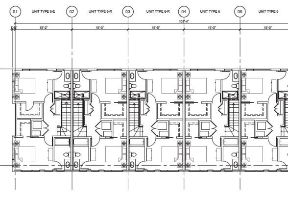
04 THIRD FLOOR PLAN DP20-09-01 1/8" = 1'-0"
