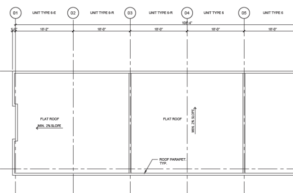
05 ROOF PLAN DP20-09-01 1/8" = 1'-0"
