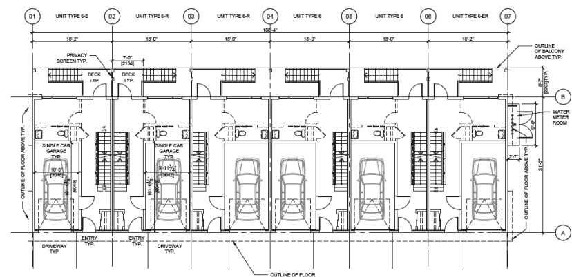
02 GROUND FLOOR PLAN DP20-09-01 1/8" = 1'-0"
